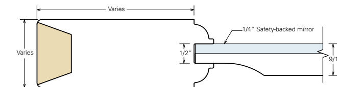
Sample cross section (one-sided mirror door)
